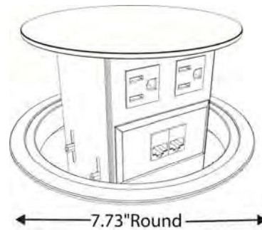
Concept Unit with Round Top and Trim Kit.
