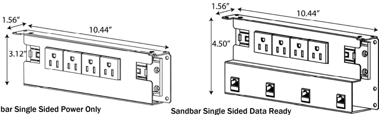
Sandbar Single Sided Data Ready
