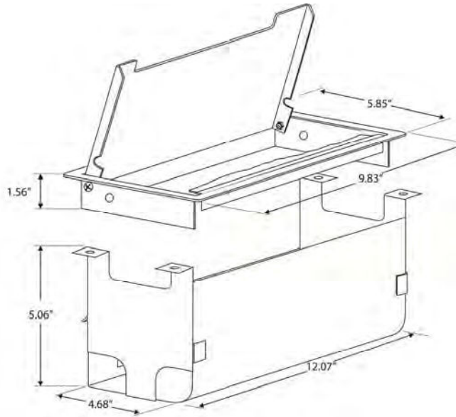
Large Hide It Kit:
