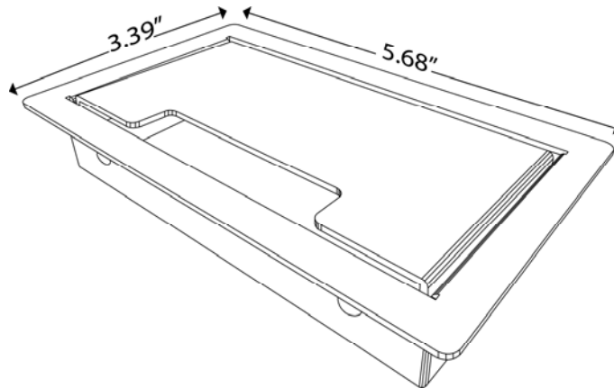
(Flush Grommet Shown, dimensions are the same for all Villa Grommets)
